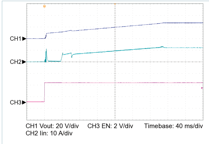
Figure 15 — Startup from EN, V_{IN} = 28\text{ V} , C_{OUT\_EXT} = 10000\text{ }\mu\text{F} , R_{LOAD} = 2.450\text{ }\Omega
