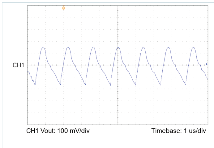
Figure 17 — Output voltage ripple, V_{IN} = 28\text{ V} , V_{OUT} = 28.0\text{ V} , C_{OUT\_EXT} = 1000\text{ }\mu\text{F} , R_{LOAD} = 2.450\text{ }\Omega
