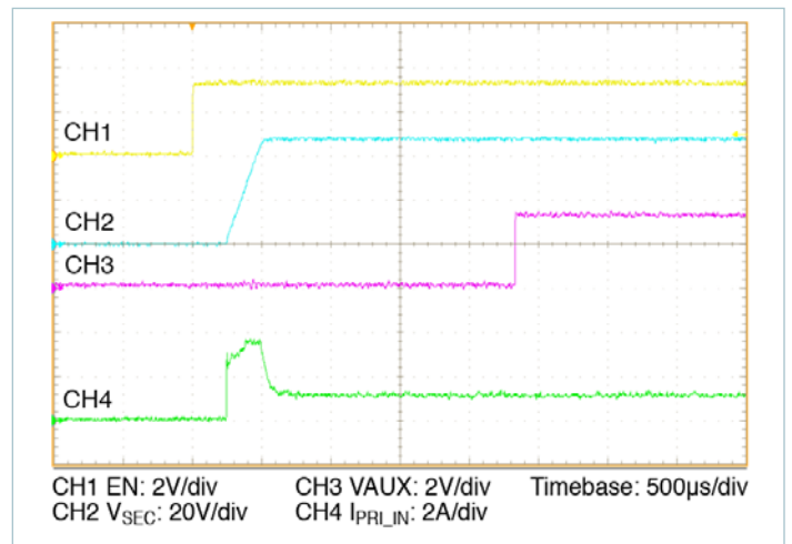
Figure 18 — Start up from application of EN with pre-applied V_{PRI\_DC} = 380V , 50% I_{SEC\_DG} , 100% C_{SEC\_OUT\_EXT}
