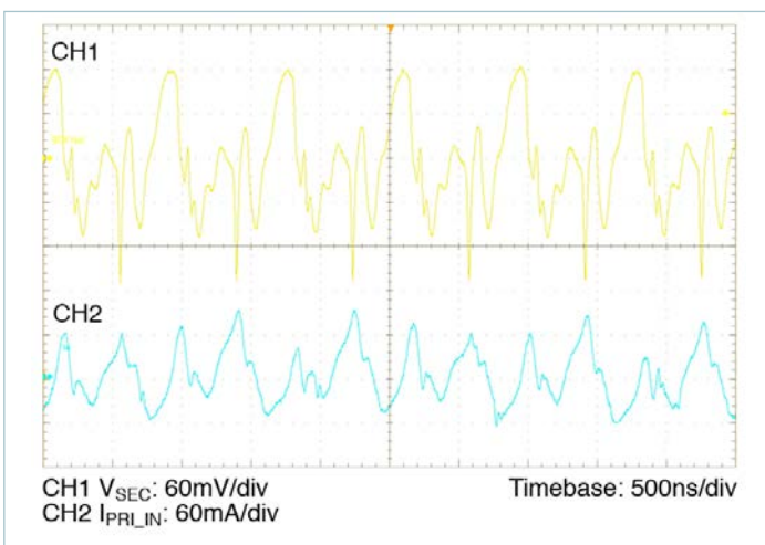
Figure 14 — Full load ripple, 270μF C_{PRI\_IN\_EXT} ; No external C_{SEC\_OUT\_EXT} . Board mounted module, scope setting: 20MHz analog BW
