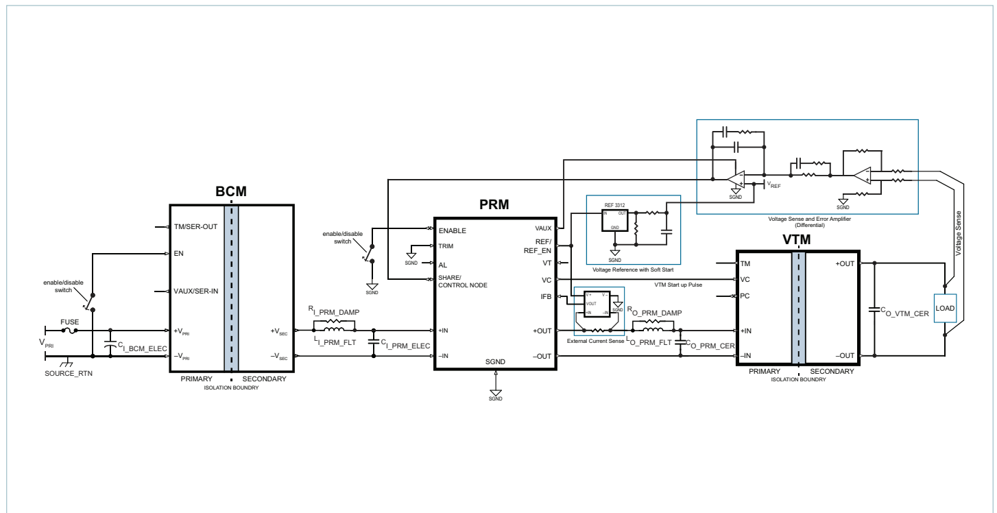
BCM6123xD1E5116yzz + PRM + VTM, Remote Sense Configuration
