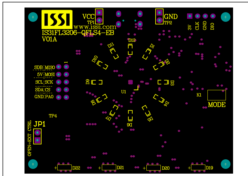
Figure 4: Board Component Placement Guide - Top Layer
