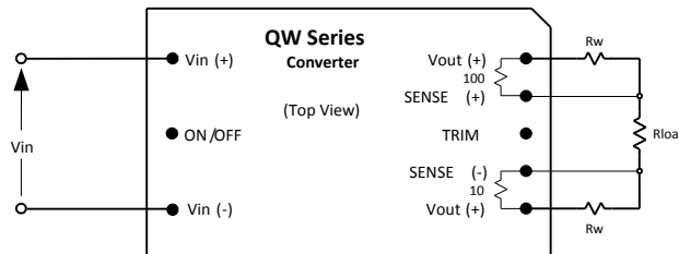
Figure 2. Remote sense circuit configuration
