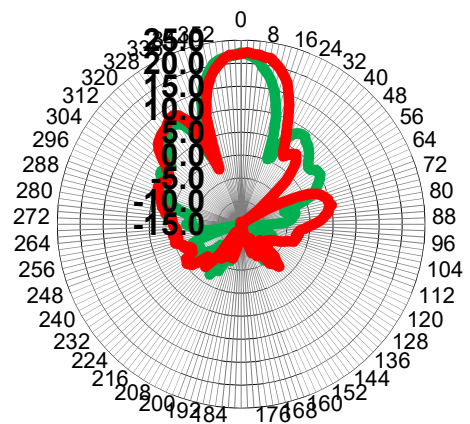
Antenna Pattern
