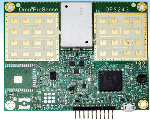
OPS243 Sensor
