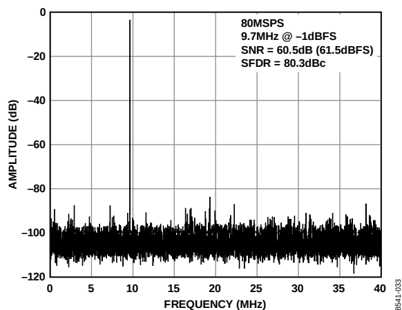
Figure 4. AD9609-80 Single-Tone FFT with f_{IN} = 9.7 MHz
