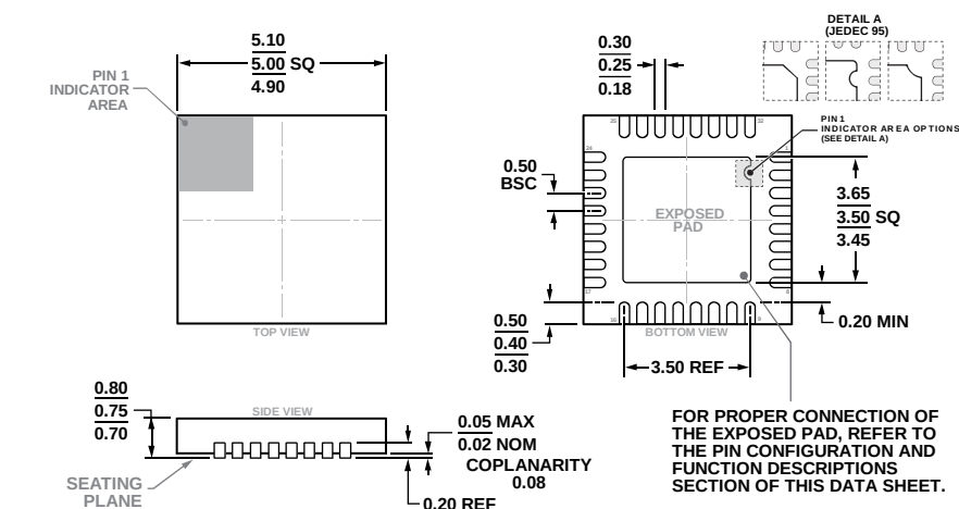
Figure 55. 32-Lead Lead Frame Chip Scale Package [LFCSP] 5 mm x 5 mm Body and 0.75 mm Package Height (CP-32-11)
