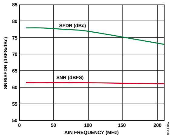
Figure 10. AD9609-80 SNR/SFDR vs. Input Frequency (AIN) with 2 V p-p Full Scale
