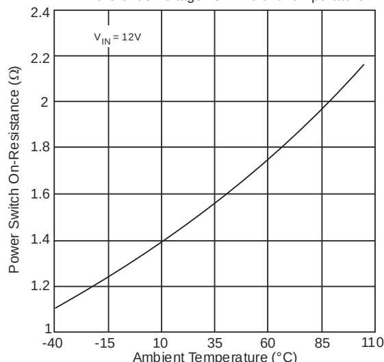
Power Switch On-Resistance vs. Ambient Temperature
