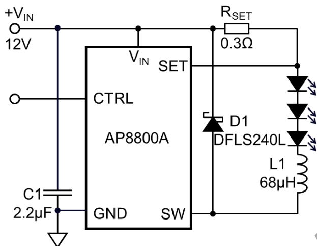
Figure 1 Typical Configuration
