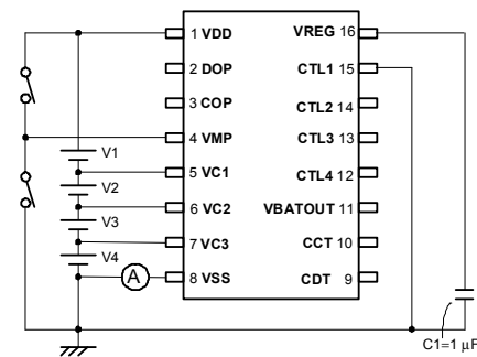
Test circuit 1
