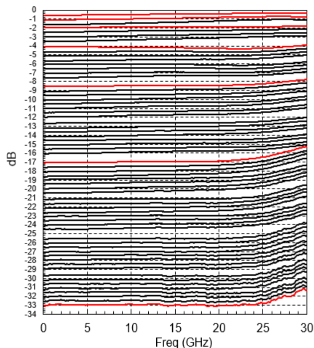
Relative Attenuation (normalized S21) @ +25°C
