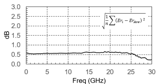
RMS Error vs. Frequency (mean) @ +25°C
