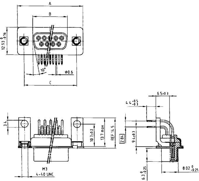
Socket connector
