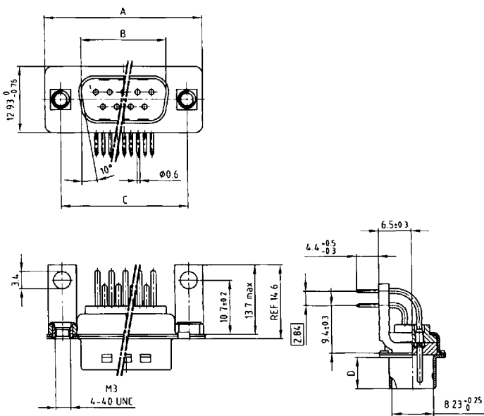
Plug connector
