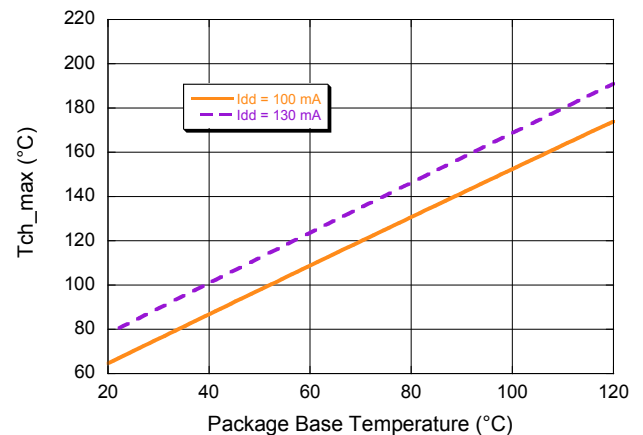
T_{ch}(\text{max.}) vs. Package Base Temperature, V_{DD} = 4\text{ V}
