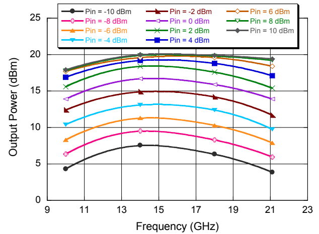
Output Power vs. Frequency, V_D = 4\text{ V} , 100 mA
