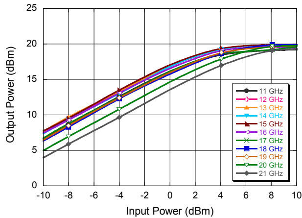
Output Power vs. Input Power, V_D = 4\text{ V} , 100 mA
