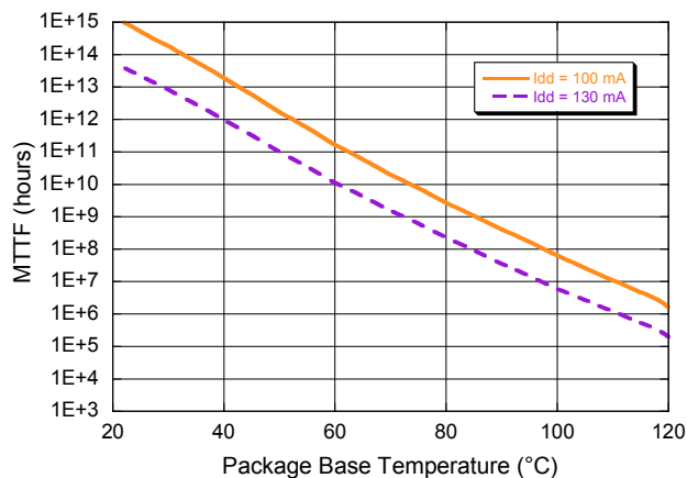
MTTF Hours vs. Package Base Temperature, V_{DD} = 4\text{ V}
