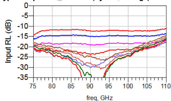
Typical Input Return Loss (dynamic range)
