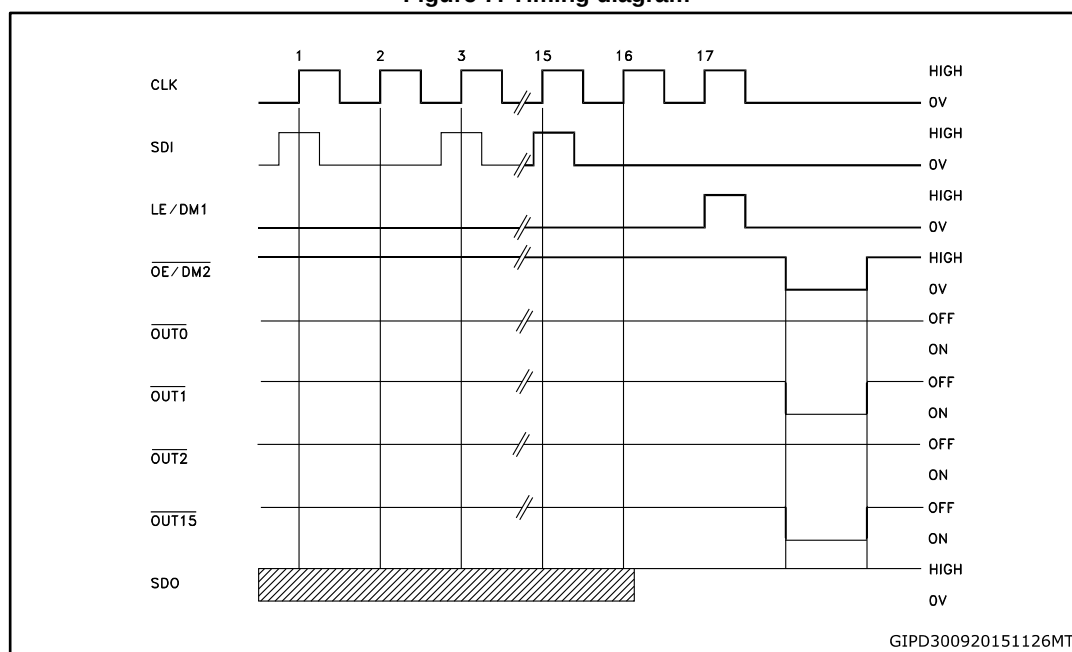
Figure 7: Timing diagram
