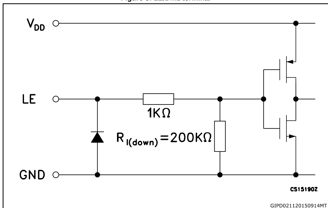
Figure 3: LE/DM1 terminal
