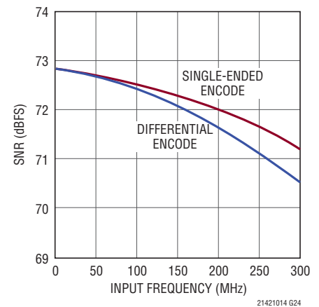
LTC2141-14: SNR vs Input Frequency, -1\text{dBFS} , 105\text{Mps} , 2V Range
