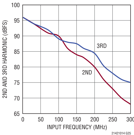
LTC2141-14: 2nd, 3rd Harmonic vs Input Frequency, -1\text{dBFS} , 40\text{Mps} , 2V Range
