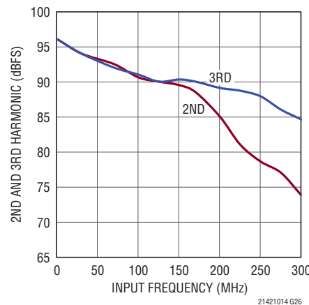
LTC2141-14: 2nd, 3rd Harmonic vs Input Frequency, -1\text{dBFS} , 40\text{Mps} , 1V Range
