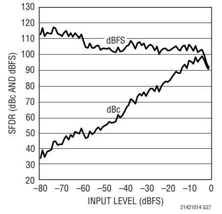
LTC2141-14: SFDR vs Input Level, f_{IN} = 70\text{MHz} , 40\text{Mps} , 2V Range
