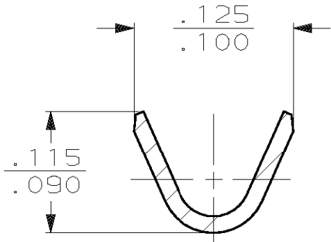
SECTION B-B SCALE 10:1
