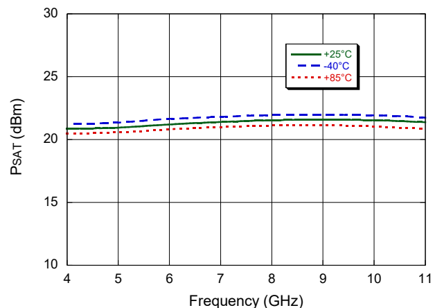
Saturated Output Power, 4 V, 130 mA
