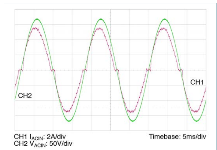
Figure 12 — Typical line current waveform, V_{IN} = 120\text{V} , 60Hz I_{OUT} = 8.3\text{A} , C_{OUT} = 10,000\mu\text{F}
