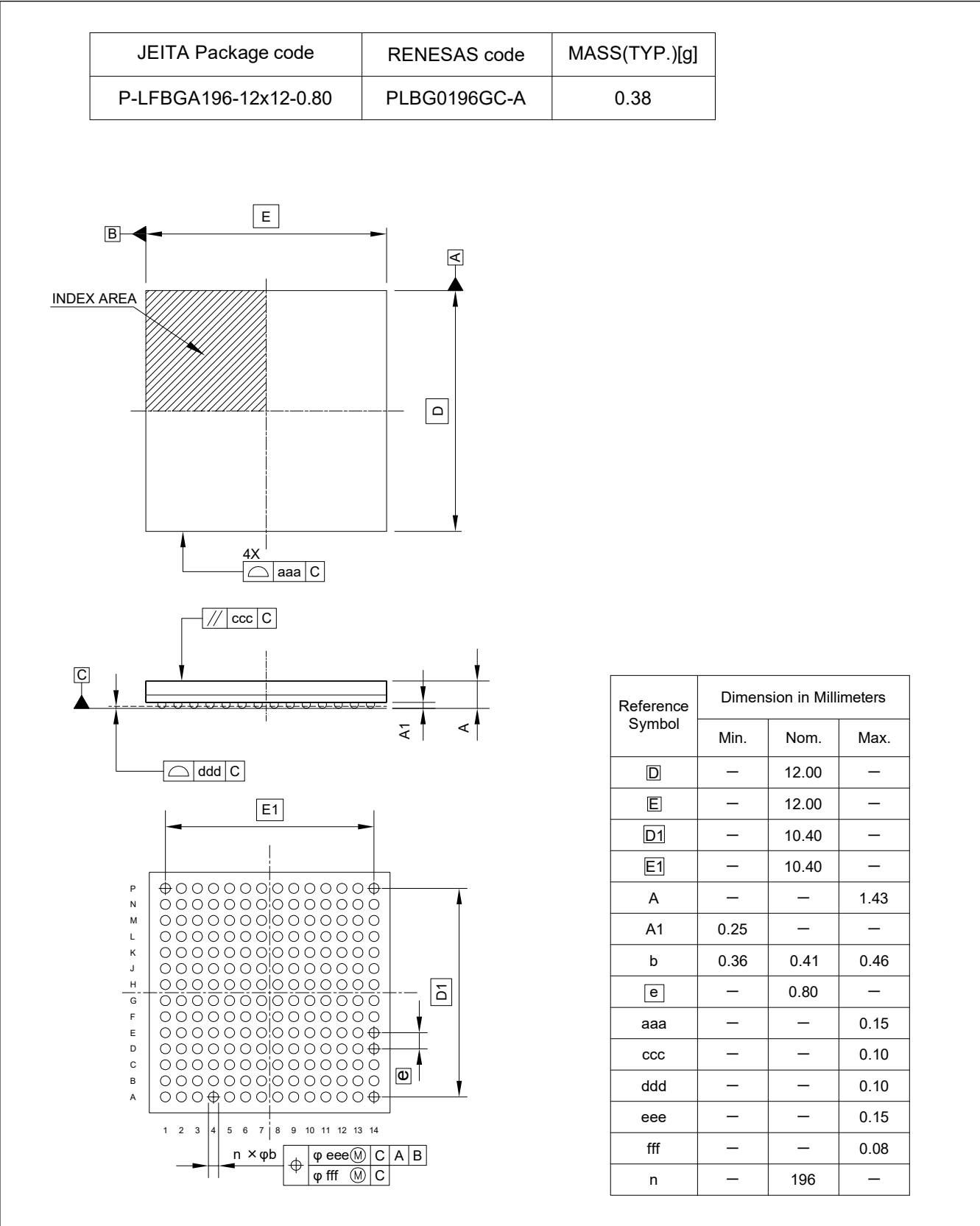
Figure 1.1 196-pin FBGA
