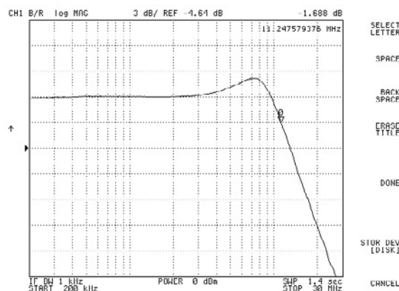
Figure 9. LTC6268 in a 499kΩ TIA with extra Layout Effort to Reduce Feedback Capacitance Achieves 11.2MHz BW
