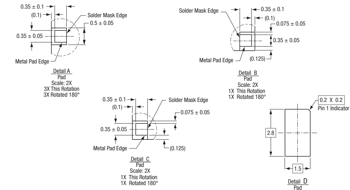
Figure 9. SKY66005-11 Package Dimensions
