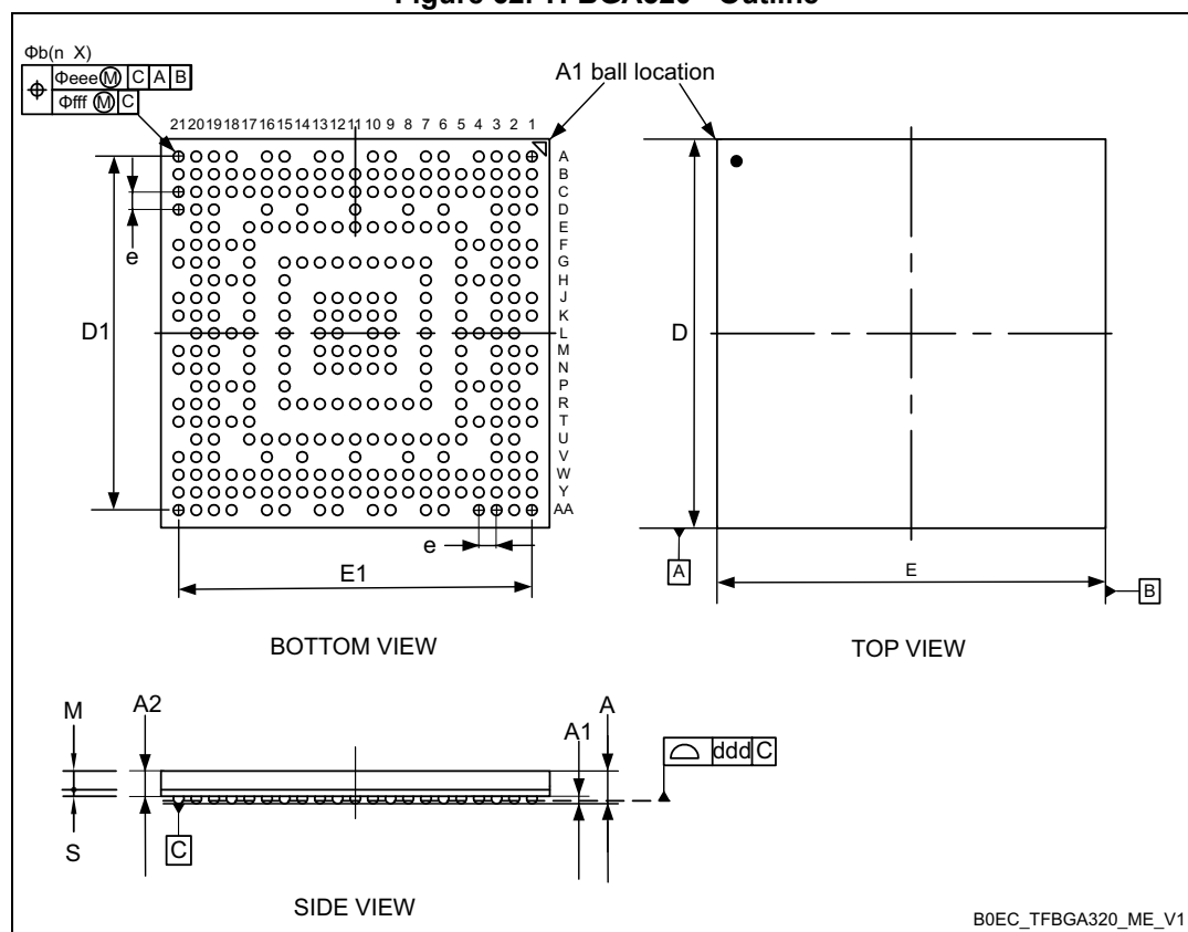
Figure 62. TFBGA320 - Outline
