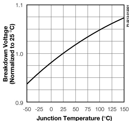
Figure 31. Breakdown vs. Temperature (Exclude INN3878C / INN3879C / INN3870C).
