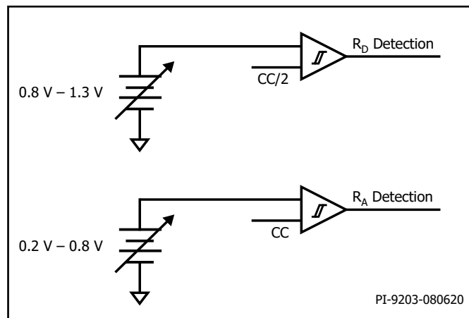
Figure 13. Type-C Detection.
