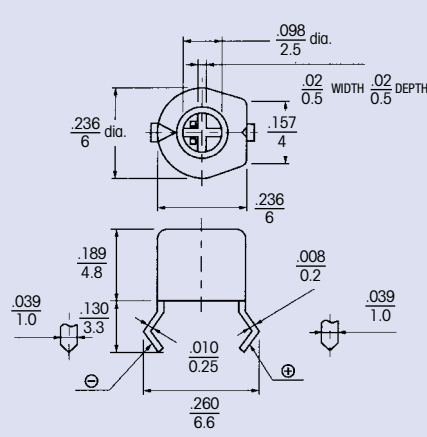
Style B (Top Adjustment)
