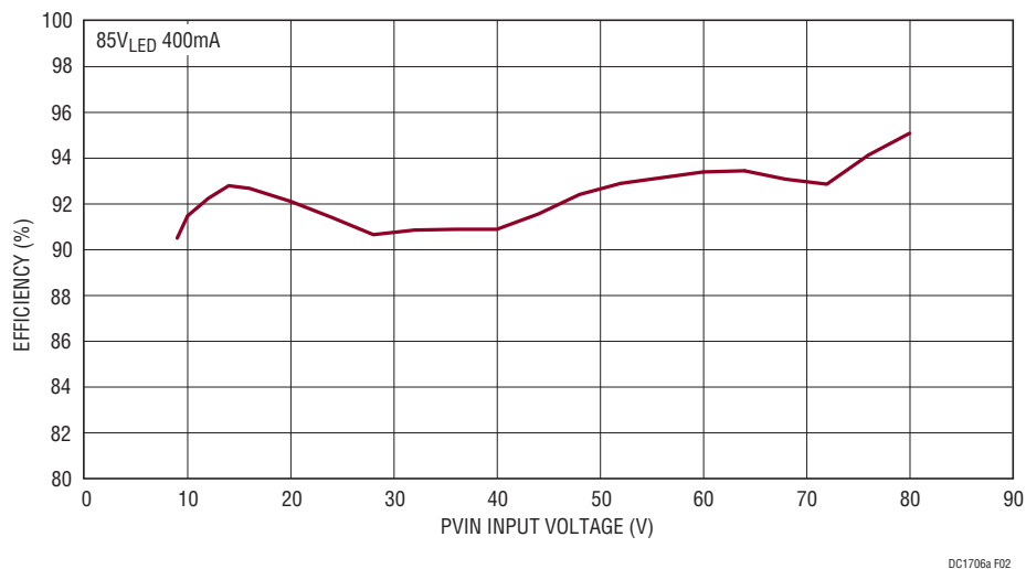
Figure 2. DC1706A Efficiency with 85V LEDs at 400mA
