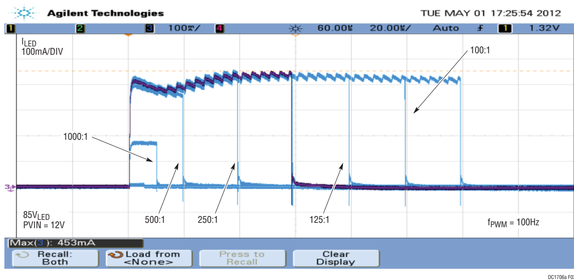
Figure 3. DC1706A 100Hz 100:1 to 1000:1 PWM Dimming Waveforms at 12V PVIN and 85V V LED
