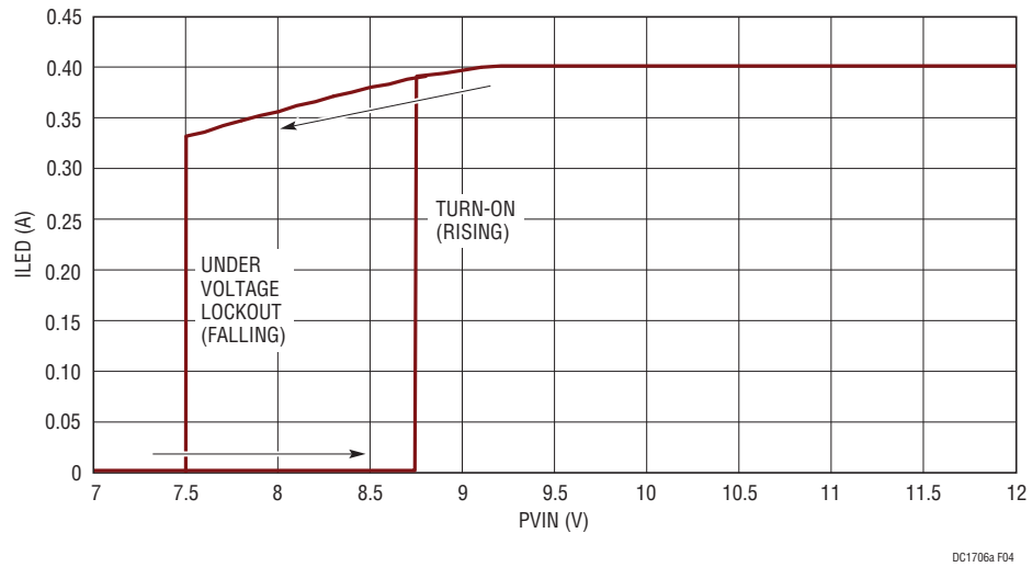
Figure 4. DC1706A CTRL LED Current Foldback at Low PV_{IN} with UVLO Falling and Rising
