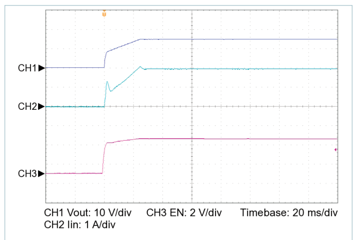
Figure 14 — Startup from EN, V_{IN} = 270\text{ V} , C_{OUT\_EXT} = 6800\text{ }\mu\text{F} , R_{LOAD} = 0.449\text{ }\Omega
