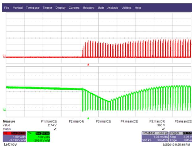
Figure 41 – 265 VAC 60 Hz, Output Short. Upper: I_{DRAIN} , 1 A / div. Lower: V_{DRAIN} , 100 V, 10 ms / div.
