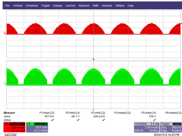
Figure 22 – 90 VAC 60 Hz, Full Load. Upper: I_{DRAIN} , 500 mA / div. Lower: V_{DRAIN} , 50 V, 5 ms / div.
