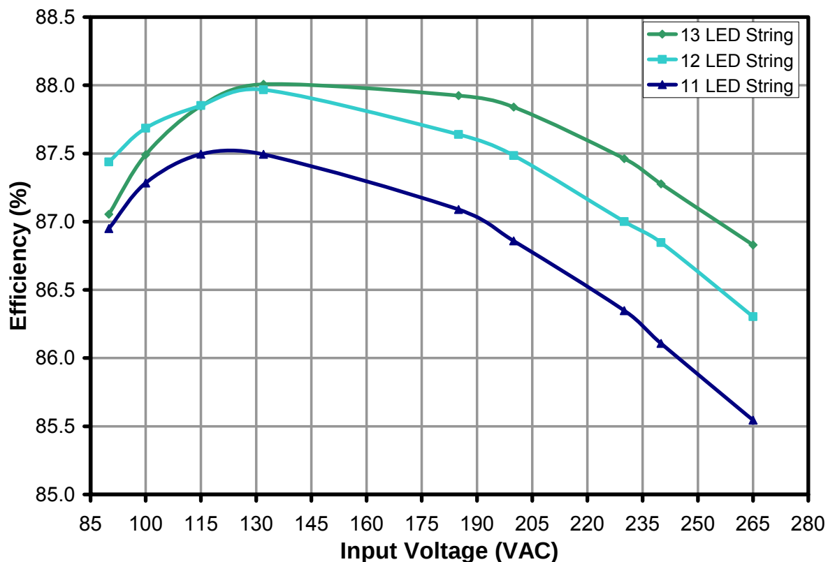
Figure 12 – Efficiency vs. Load and Input Voltage.
