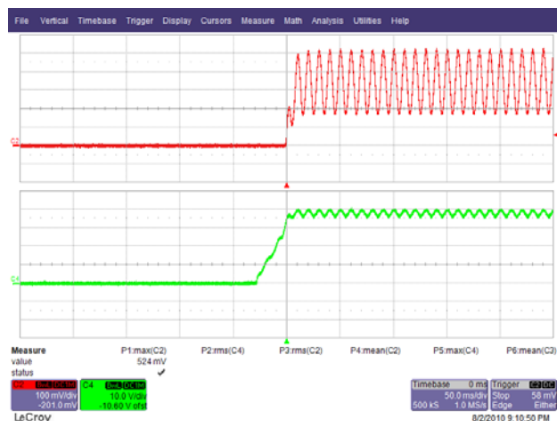
Figure 38 – 265 VAC 50 Hz, Output Rise. Upper: I_{OUT} , 100 mA / div. Lower: V_{OUT} , 10 V, 50 ms / div.
