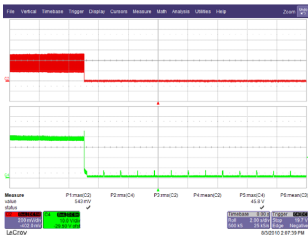
Figure 43 – 265 VAC 60 Hz, Open Load. CH2: I_{OUT} , 200 mA / div. CH4: V_{OUT} , 10 V, 1 s / div.
