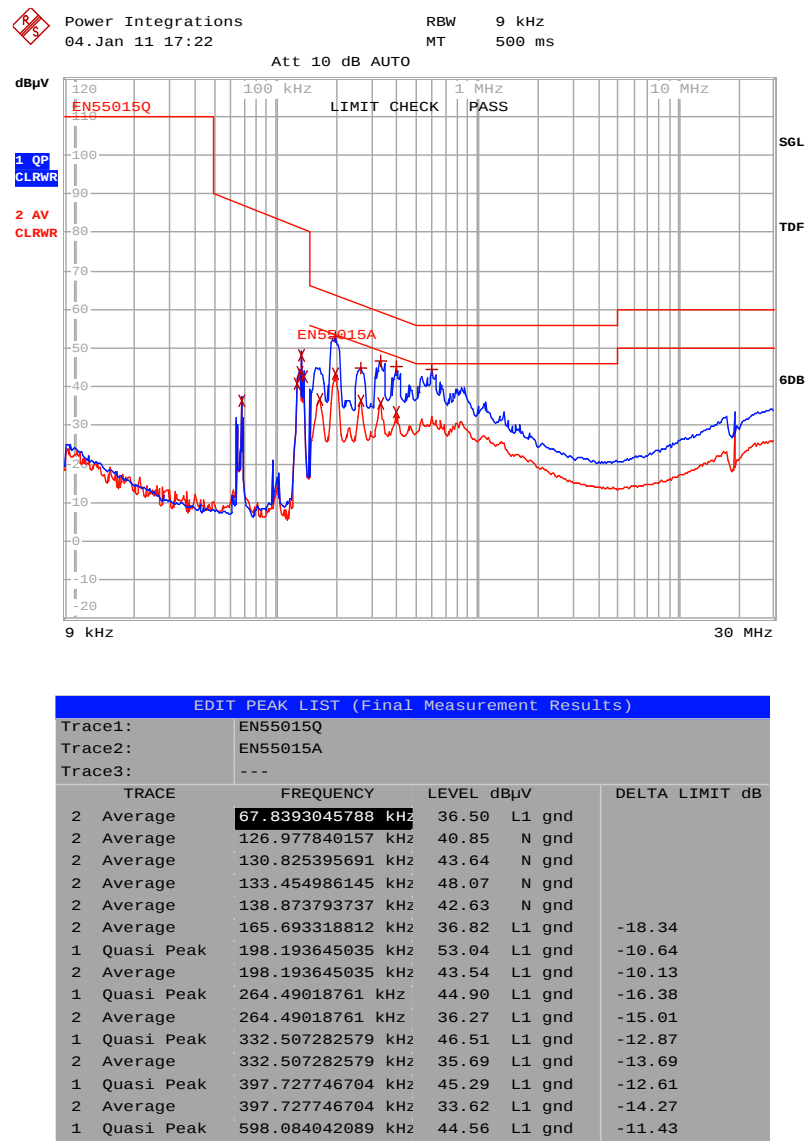
Figure 48 – Conducted EMI, ~36 V Load, 115 VAC, 60 Hz, and EN55022 B Limits.
