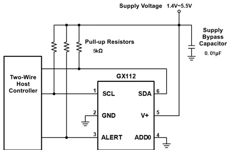
Figure 9. Typical Connections of the GX112
