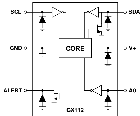
Figure 2. GX112 Internal ESD Equivalent Circuit
