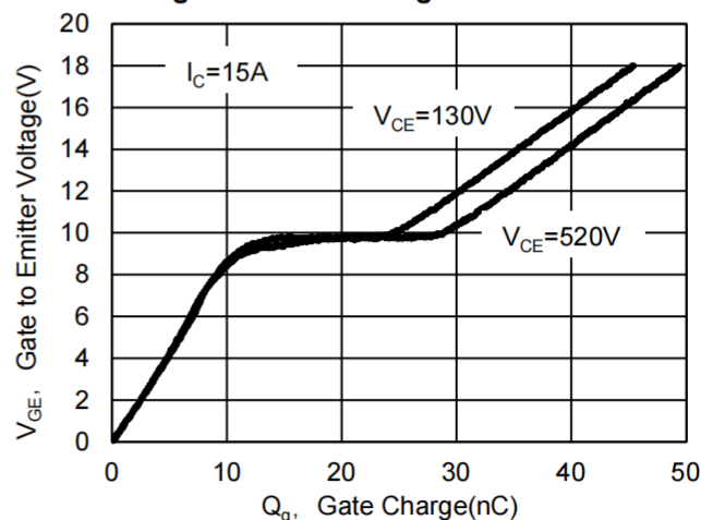
Figure 6. Gate-Charge Characteristics
