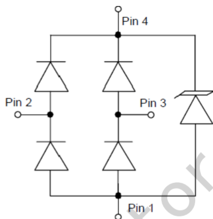
Circuit Diagram
