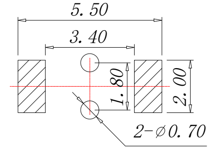
PCB.WELDING DRAWING
