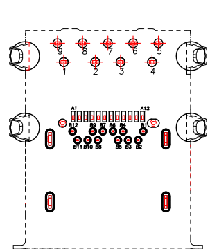
CONNECTOR EDGE(TOP VIEW)
