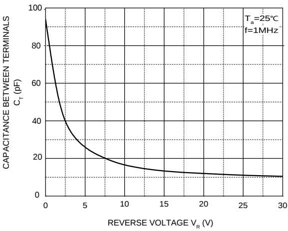
FIG.4-TYPICAL JUNCTION CAPACITANCE
