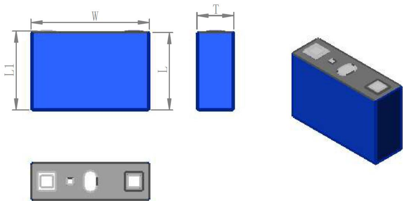
电芯尺寸Celldimension
