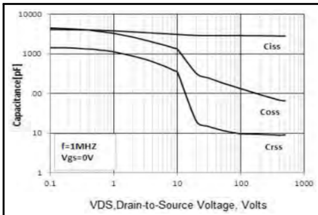
Figure 5: Capacitance Characteristics
