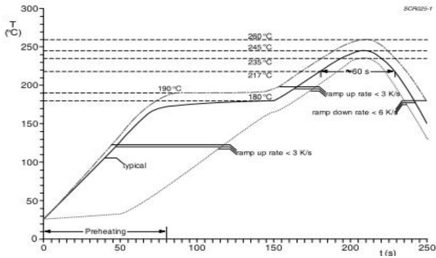
Fig7: Infrared soldering forced air convection reflow soldering-temperature/time profile for SnAgCu solders
