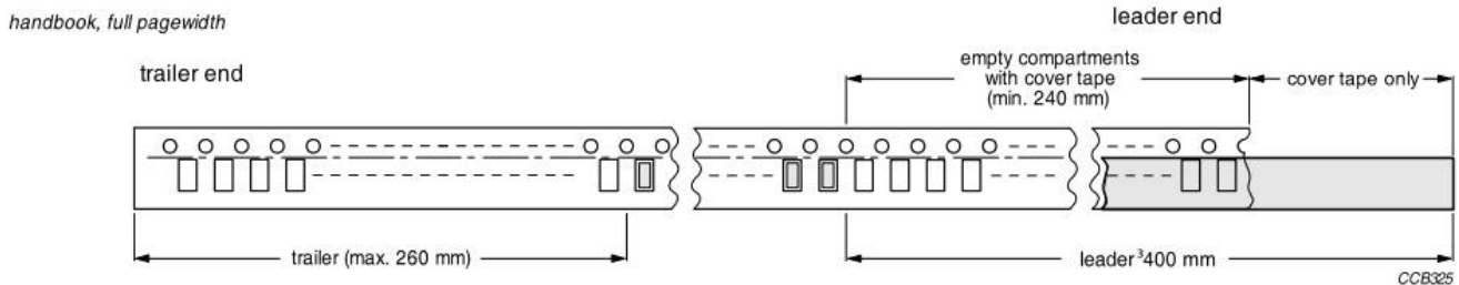
Fig12: Peel-off force
