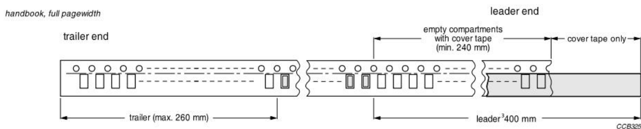
Fig11: Leader/trailer tape
