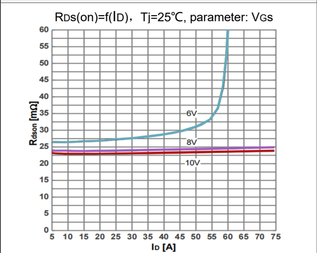
Figure 6. Typ. drain-source on-state resistance
