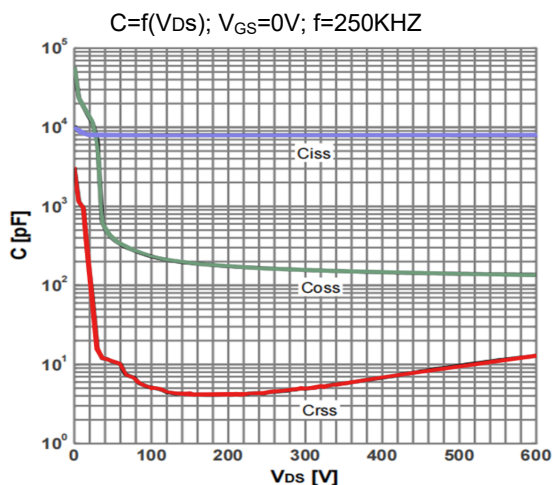
Figure 12. Typ. capacitances
