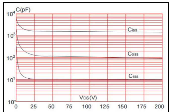
Figure 6: Capacitance Characteristics
