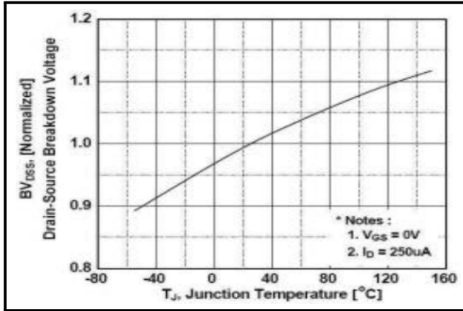
Figure 7: V_{BR(DSS)} vs. T_J
