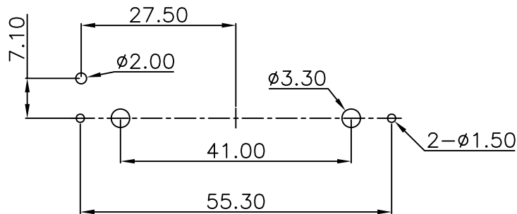
MOUNTING DETAIL
