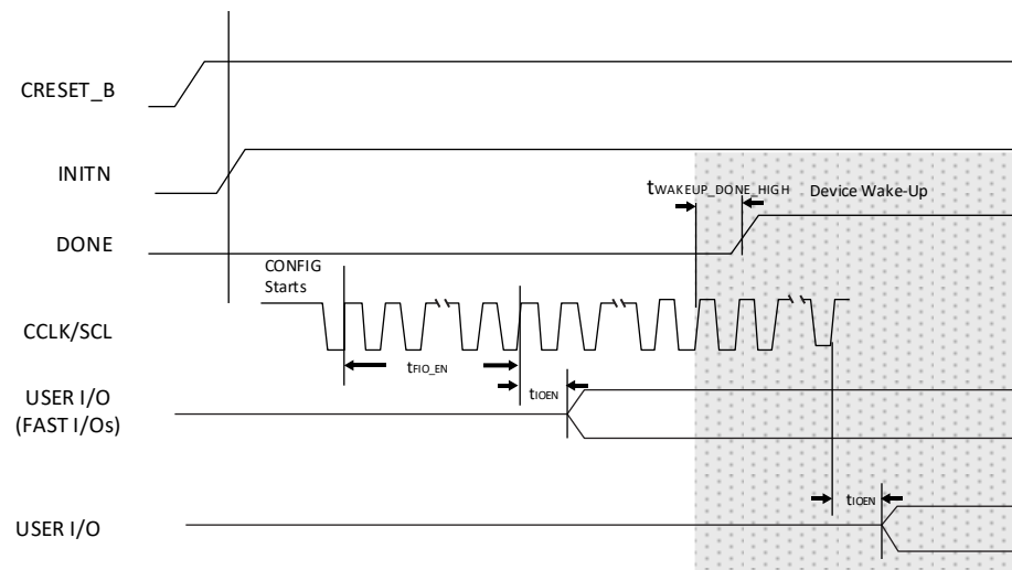
Figure 3.22. Slave SPI/I²C/I3C Wake-Up Timing
