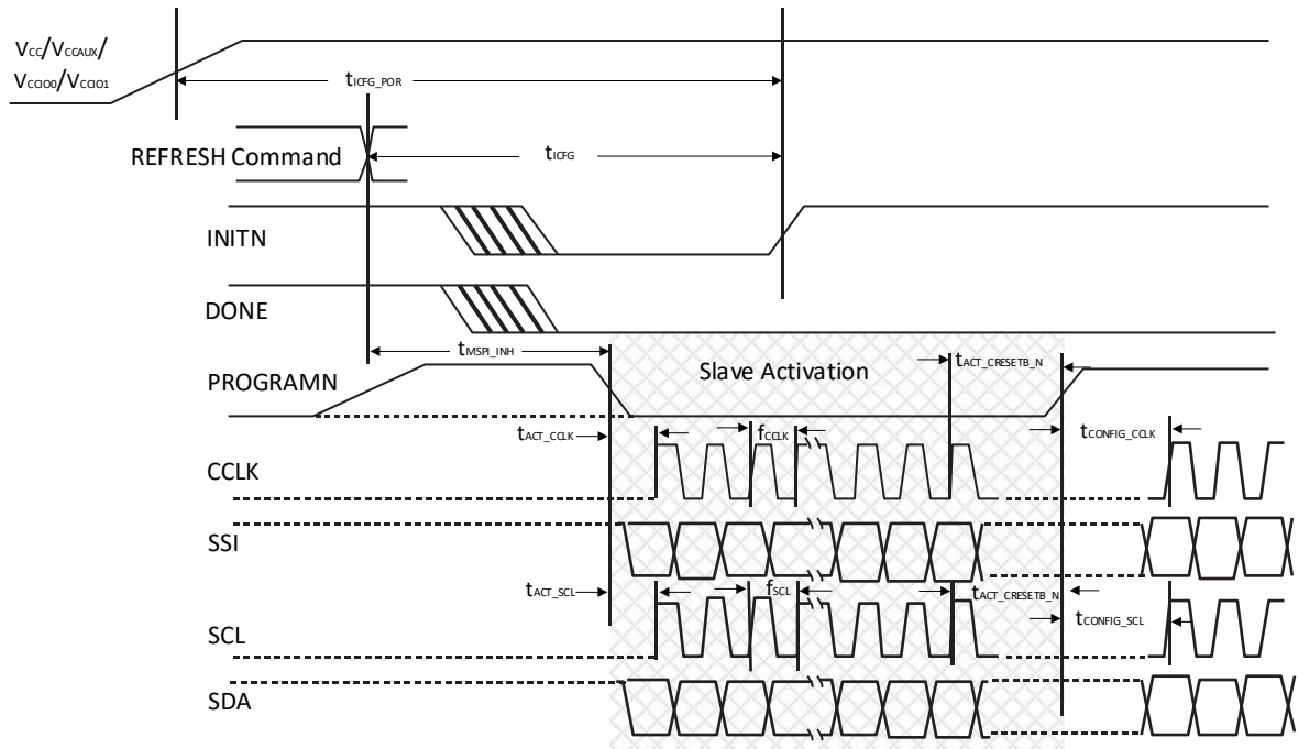
Figure 4.15. Slave SPI/I²C/I³C POR/REFRESH Timing
