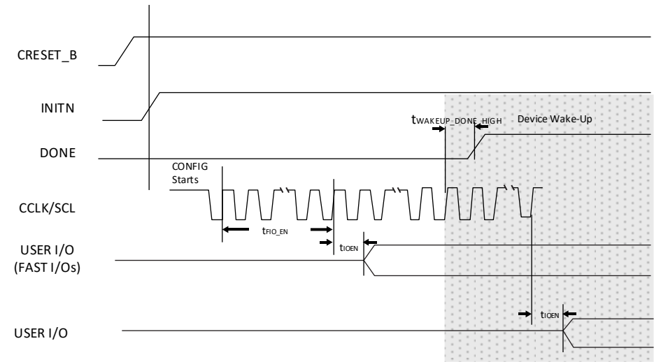
Figure 4.22. Slave SPI/I 2 C/I 3 C Wake-Up Timing
