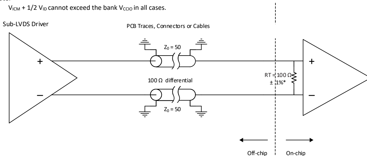
Figure 3.3. SubLVDS Input Interface
