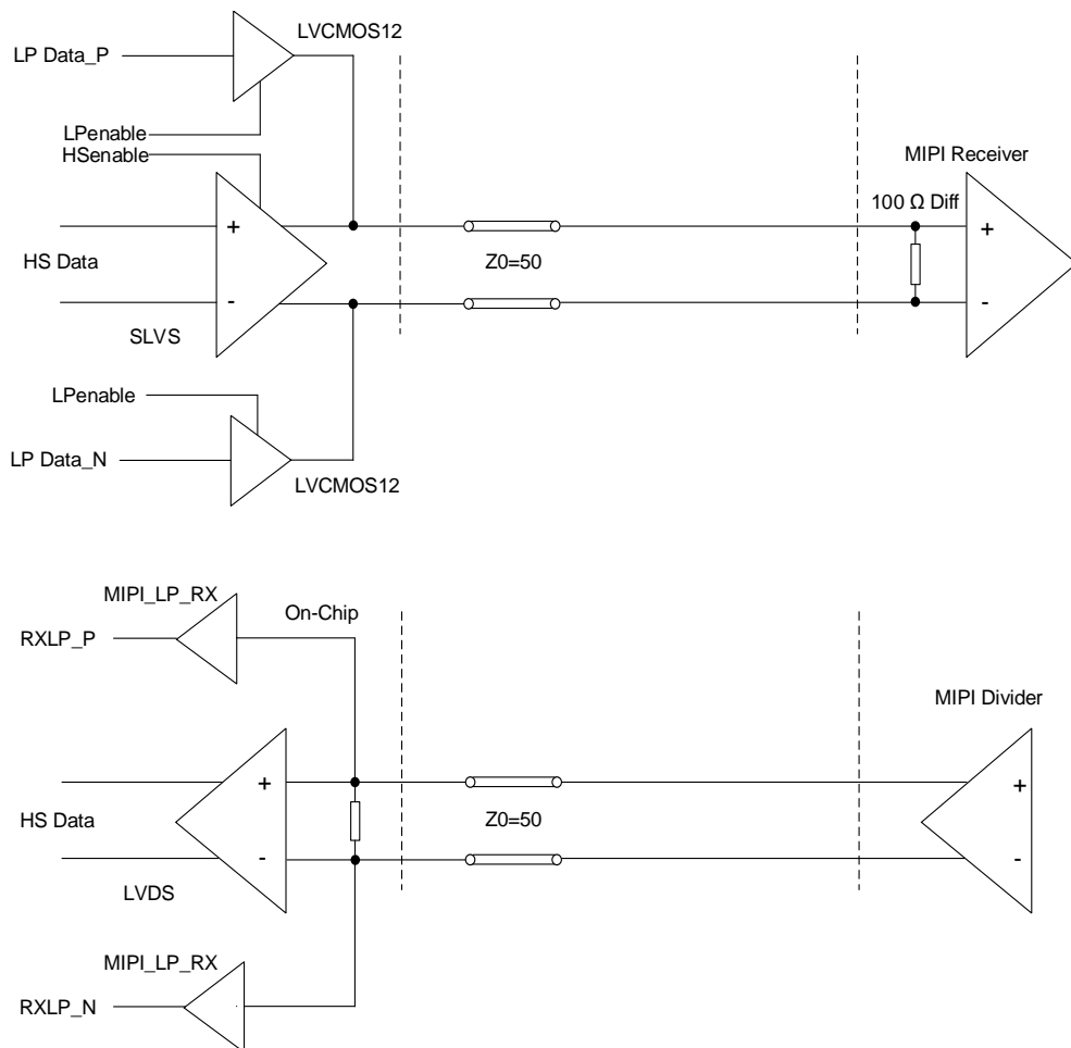
Figure 4.6. MIPI Interface
