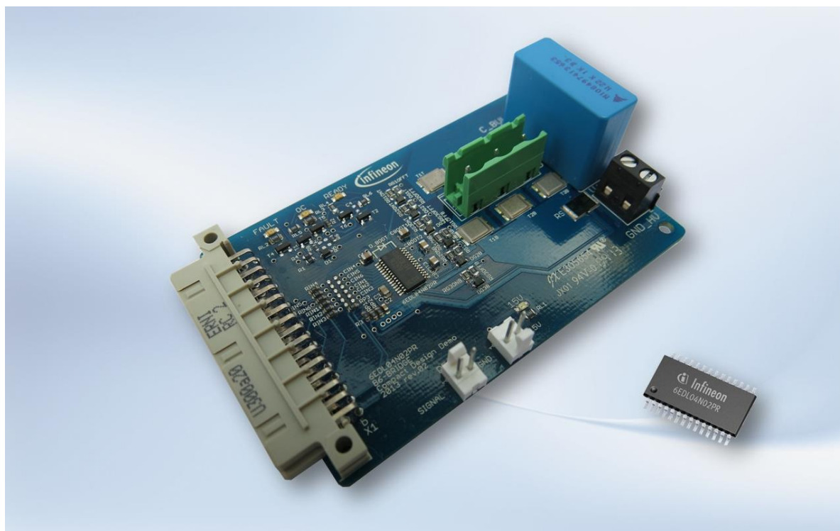
Figure 2-1 top view of the EVAL_6EDL04N02PR
