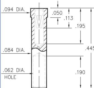
5295-0-19-XX-06-XX-10-0 Solder mount in .086 min. mounting hole
