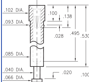
0396-0-15-XX-06-XX-10-0 Press-fit in .090 mounting hole
