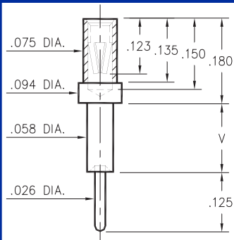
0298-X-15-XX-06-XX-10-0 Swage mount in .060 hole
