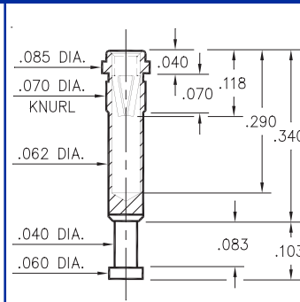
8864-0-15-XX-06-XX-10-0 Press-fit in .067 mounting hole
