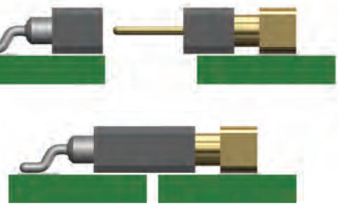
Z-Bend Style SIP Socket HSMT (.100" Grid)
