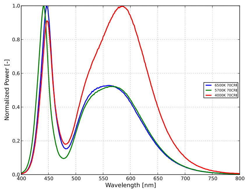
Figure 2. Typical normalized power vs. wavelength for LUXEON V at 1400mA, T j =85°C.
