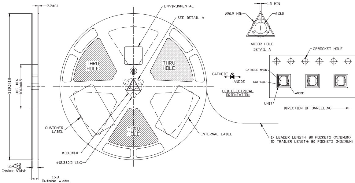
Figure 14. Reel dimensions for LUXEON V.
