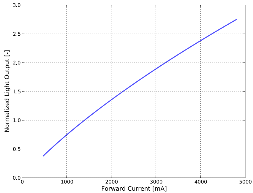
Figure 4. Typical normalized light output vs. forward current for LUXEON V at 1400mA, T j =85°C.
