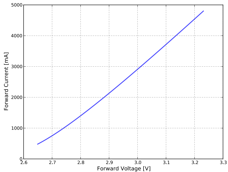
Figure 5. Typical forward current vs. forward voltage for LUXEON V at T j =85°C.
