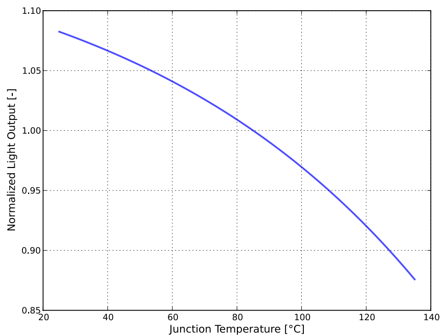
Figure 3. Typical normalized light output vs. junction temperature for LUXEON V at 1400mA, T j =85°C.
