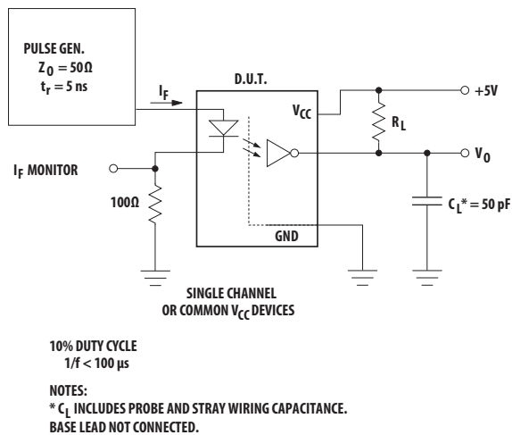
Figure 9 Switching Test Circuit
