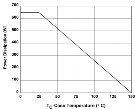
Figure 9. Maximum Power vs Case Temperature
