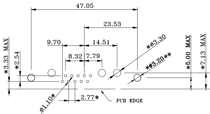
20 AMP CONFIGURATION
