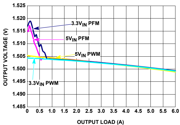
FIGURE 15. V_{OUT} REGULATION vs LOAD (1MHz, V_{OUT} = 1.5\text{V} )
