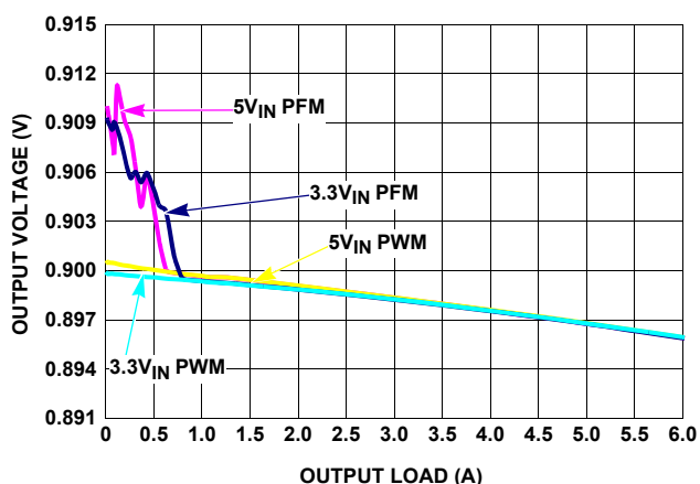
FIGURE 13. V_{OUT} REGULATION vs LOAD (1MHz, V_{OUT} = 0.9\text{V} )
