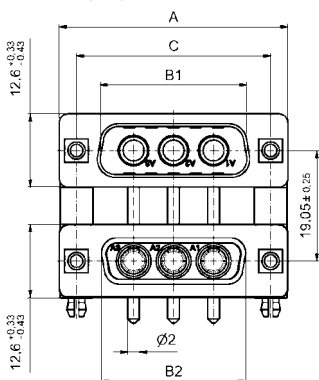
Mounting style: PCB clip and 4-40 UNC threaded insert
