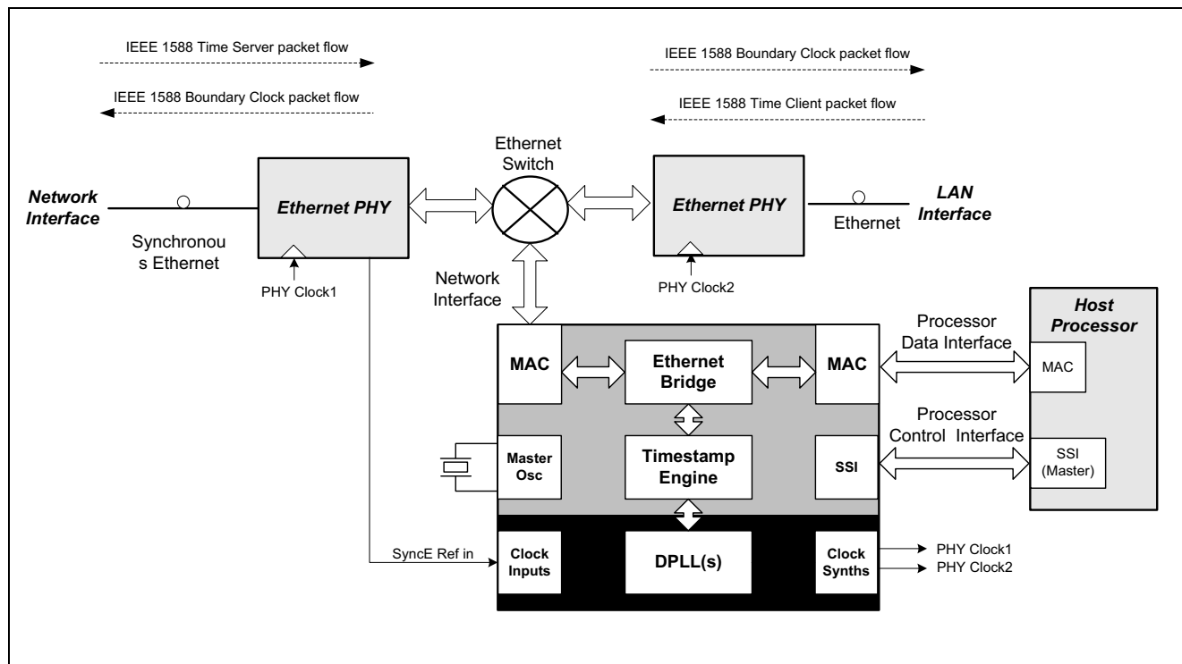
Figure 11 - ZL30314 Boundary Clock
