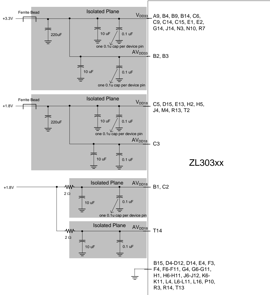
Figure 7 - Power Supply Decoupling for the ZL30314
